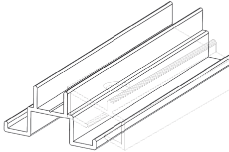
RE15 Top Rail Adaptor for RE1
